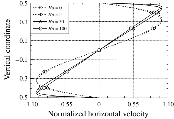
FIGURE 10. Vertical profiles of the normalized horizontal velocity at mid-length of the cavity. Results obtained by numerical simulation in the rigid-rigid case for buoyancy effect ( Gr = 2 \times 10^4 ) and Ha = 0, 5, 50 and 100 .
