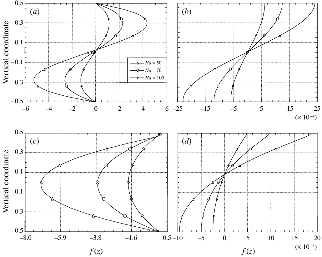
FIGURE 5. Vertical profiles of the temperature given by f(z) . Analytical solution (3.5) in the rigid-free case for Ha = 50, 70 and 100 , for buoyancy or thermocapillary effect and different thermal boundary conditions. (a) Conducting case, Gr = 10^4 , Re = 0 ; (b) insulated case, Gr = 10^4 , Re = 0 ; (c) conducting case, Gr = 0 , Re = 10^4 ; (d) insulated case, Gr = 0 , Re = 10^4 .
