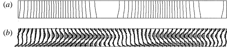
FIGURE 29. Electric characteristics for the three-dimensional longitudinal mode given in the (y, z) -plane. The iso-lines for the electric potential (a) and the electric current projection (b) are given for the perturbation at marginal state at Pr = 0.02 and Ha = 5 .
