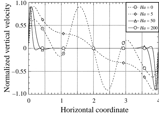
FIGURE 11. Horizontal profiles of the normalized vertical velocity at mid-height of the cavity. Results obtained by numerical simulation in the rigid-rigid case for buoyancy effect ( Gr = 2 \times 10^4 ) and Ha = 0, 5, 50 and 200 .
